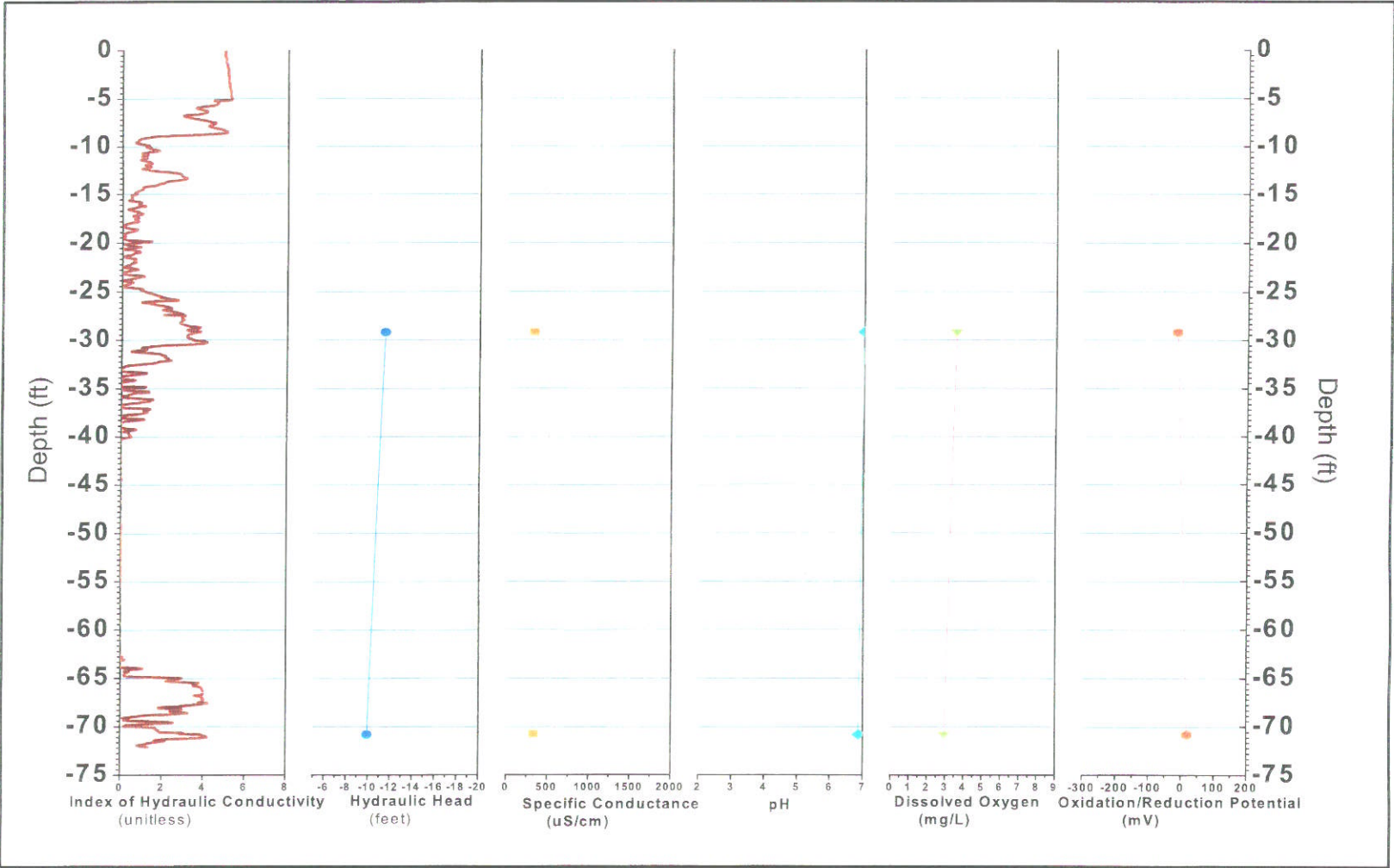
FIGURE B-237, I K RECORD AND PHYSICO-CHEMICAL PARAMETERS ERM, Wayland, Massachusetts
