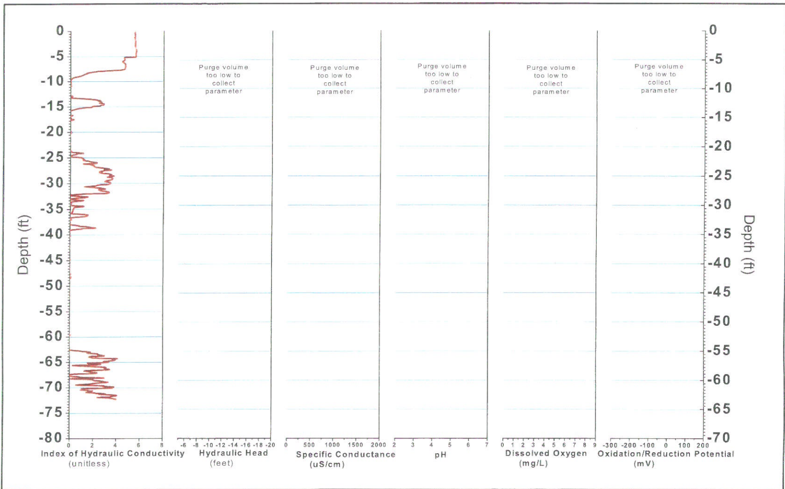
FIGURE B-239, I_K RECORD AND PHYSICO-CHEMICAL PARAMETERS ERM, Wayland, Massachusetts
