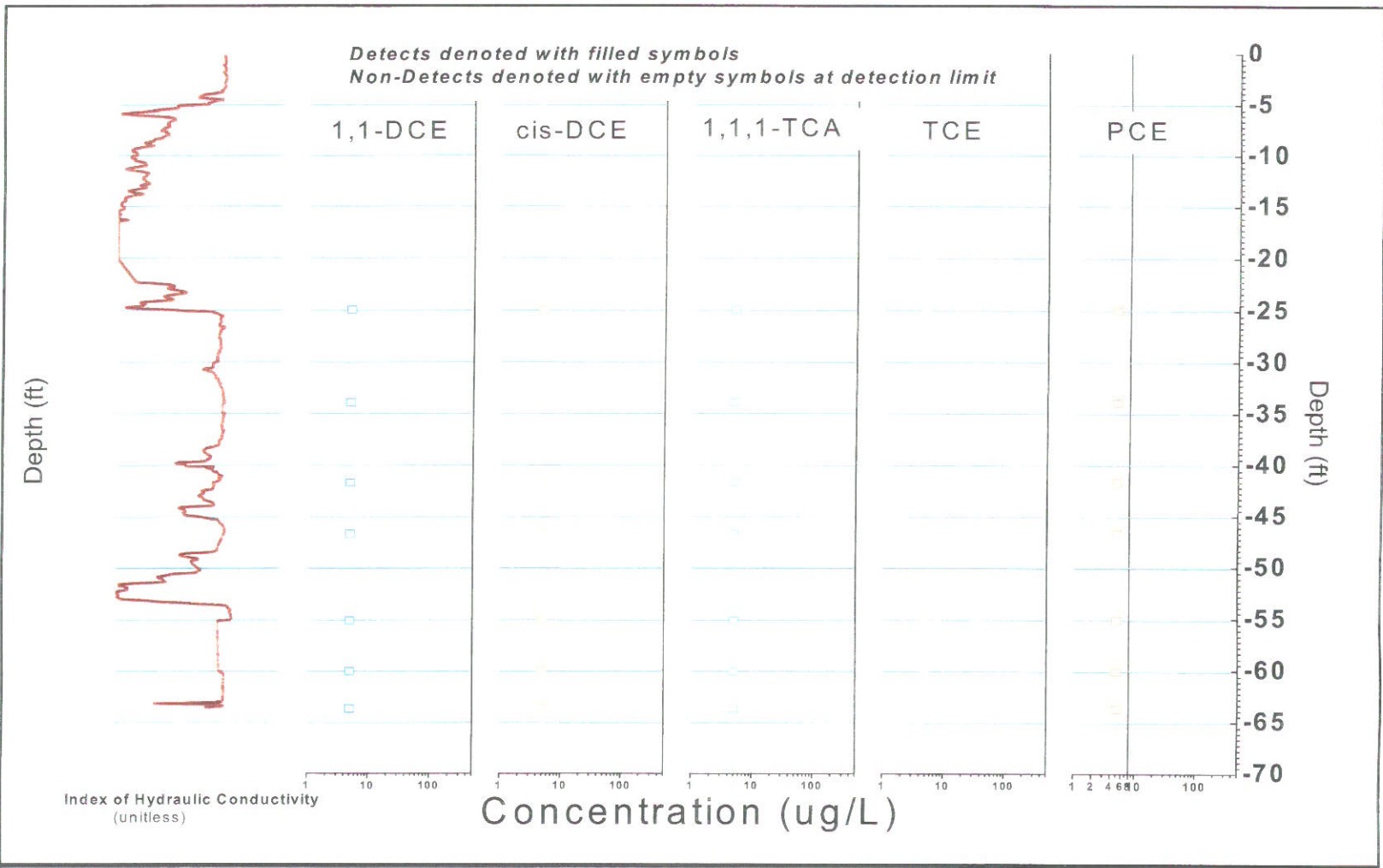
FIGURE B-236, I_k RECORD AND SELECTED VOC ANALYTICAL RESULTS ERM, Wayland, Massachusetts
