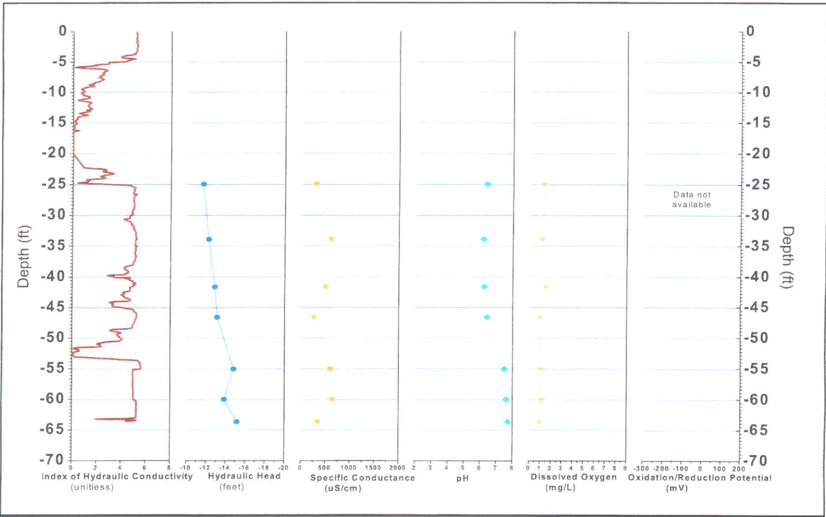
FIGURE B-236, I k RECORD AND PHYSICO-CHEMICAL PARAMETERS ERM, Wayland, Massachusetts
