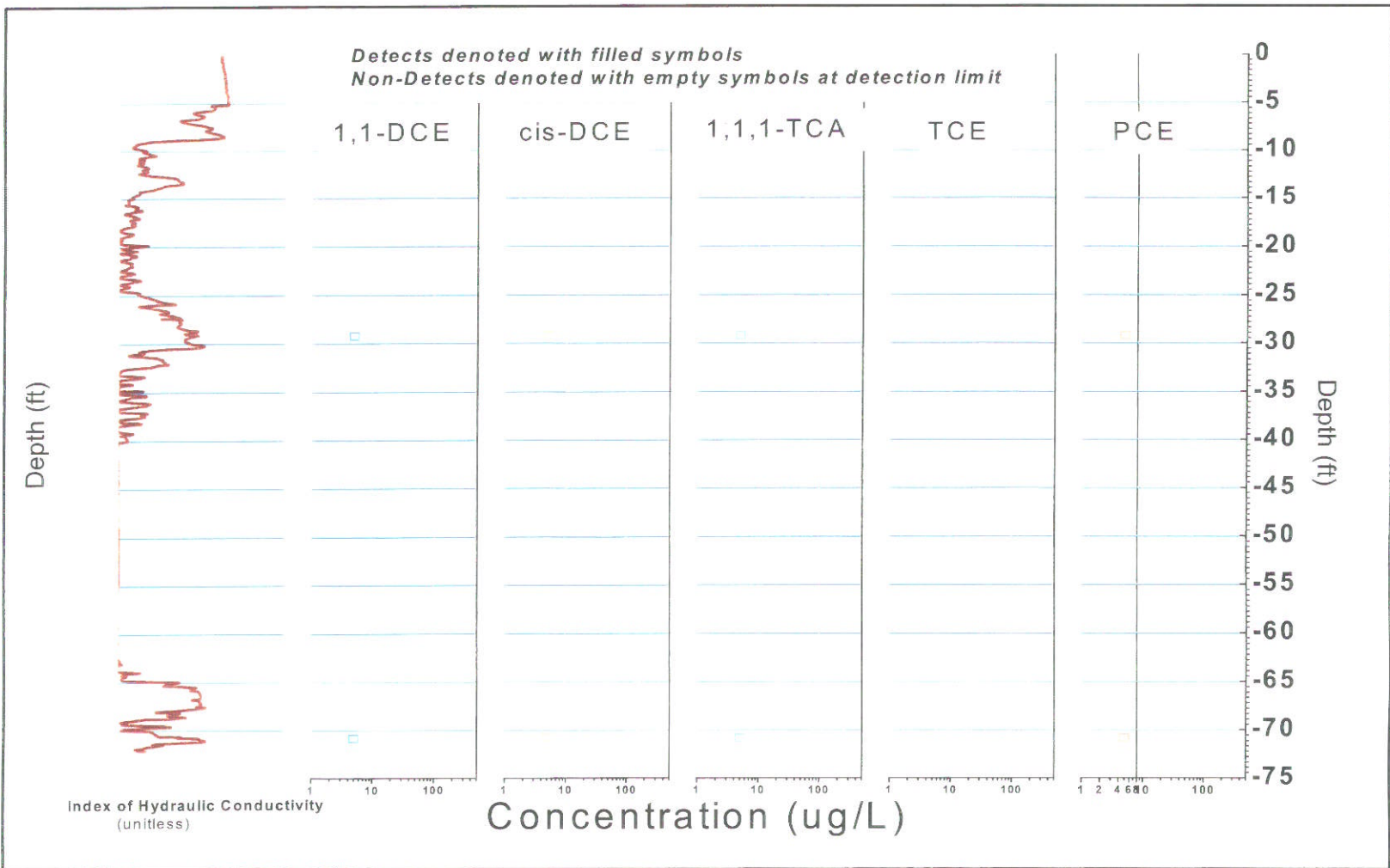
FIGURE B-237, I_k RECORD AND SELECTED VOC ANALYTICAL RESULTS ERM, Wayland, Massachusetts
