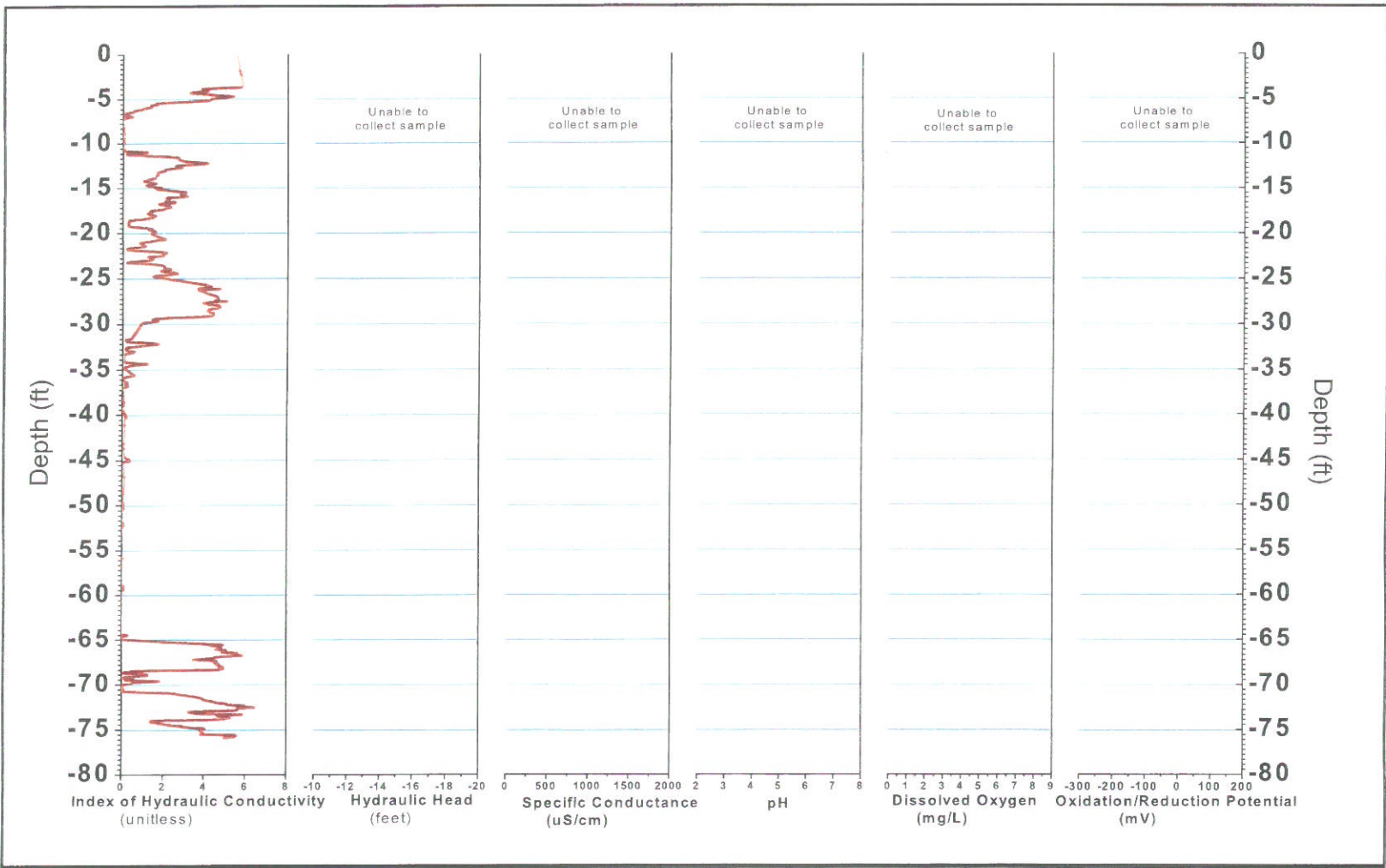
FIGURE B-238, I k RECORD AND PHYSICO-CHEMICAL PARAMETERS ERM, Wayland, Massachusetts
